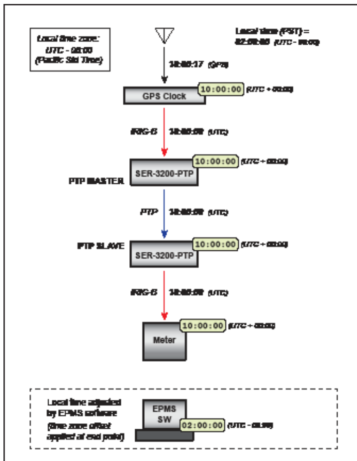
Figure 8-1. Local time adjusted at end-use point (EPMS software).
