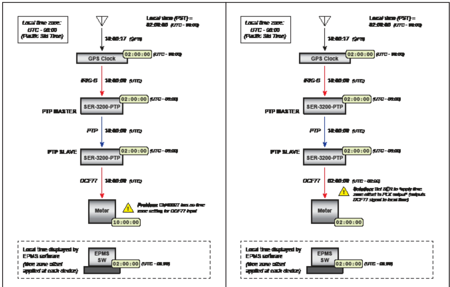
Figure 8-3. Local time adjusted at each device—except one.
