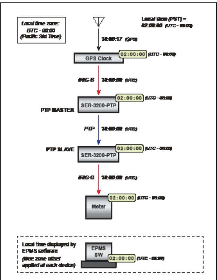
Figure 8-2. Local time adjusted at each device in system.
