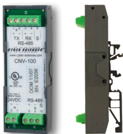
CNV-100 RS-485 2-Wire to 4-Wire Converter
